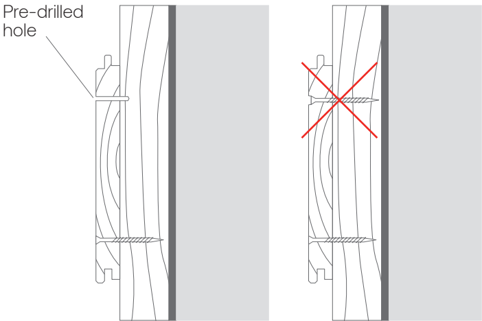
THERMORY CLADDING PROFILES FOR FASTENING WITH SCREWS ONLY:
