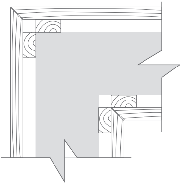
Cut the boards to a 45-degree angle.
