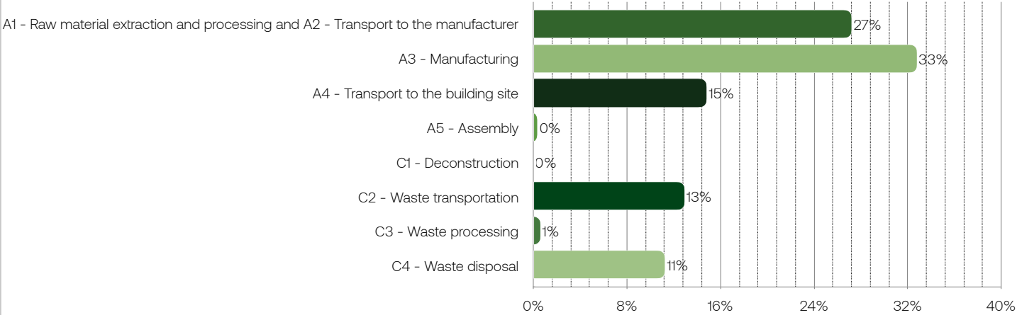
Thermally modified hardwood without surface coating
