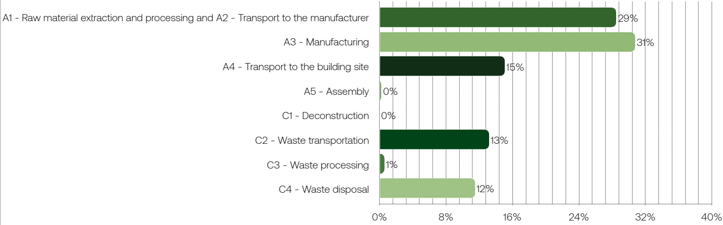
Thermally modified hardwood with surface coating
