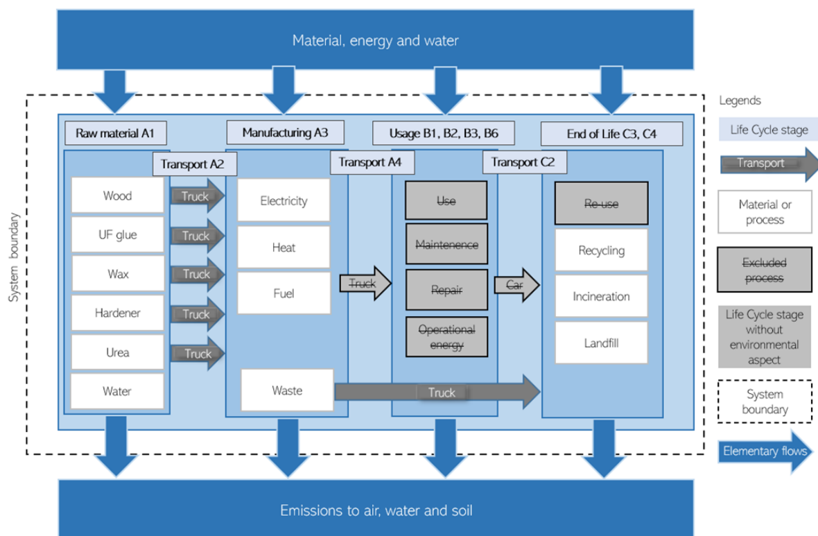
Figure 3 System diagram for P2 and P6 showing what is included in each module declared in the EPD.
