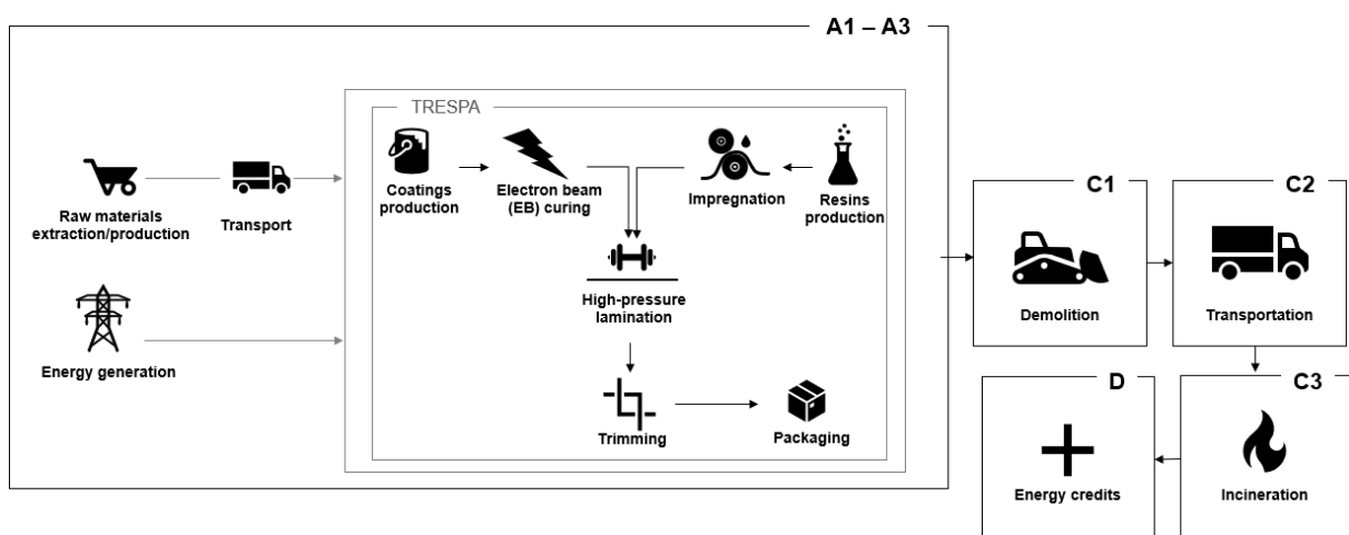
Figure 1: System boundary diagram for Trespa Meteon EDF 8mm
